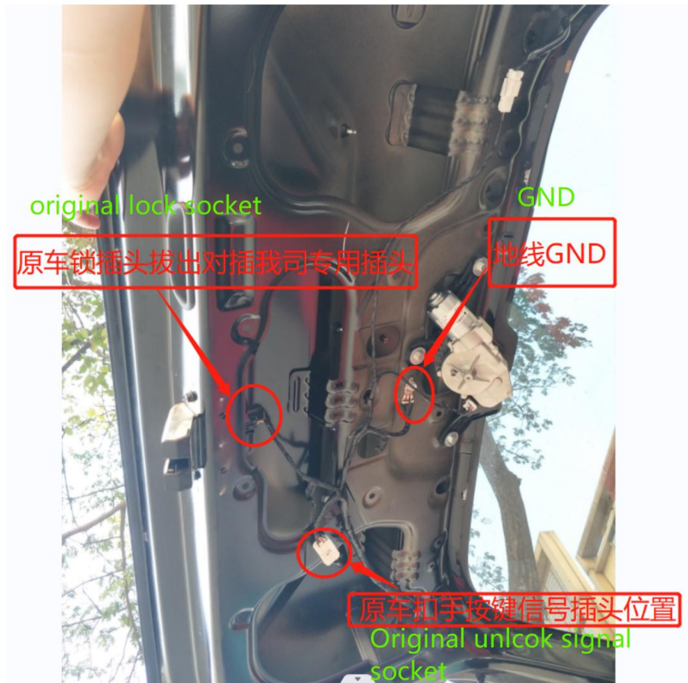
13. Original lock socket ,GND and original unclok signal socket.
