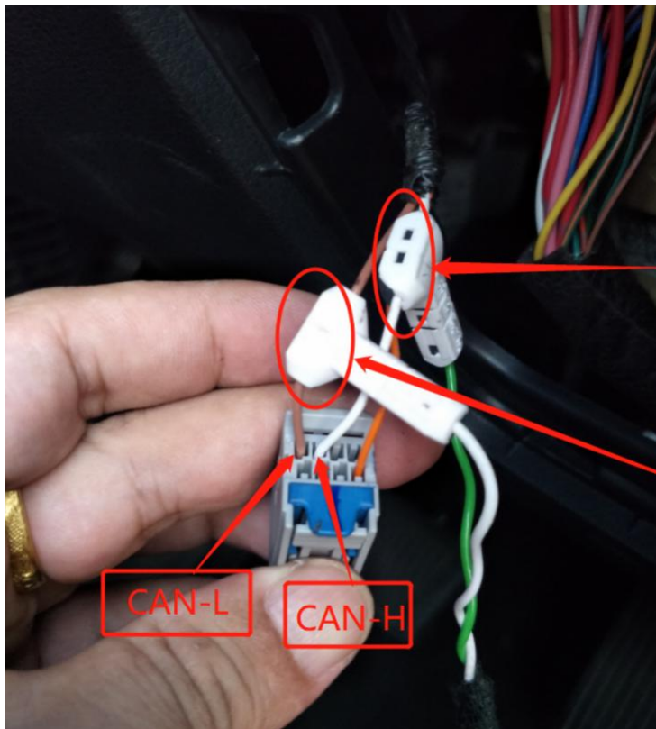
23. Factory green wire to CAN-H and factory white wire to CAN-L.
