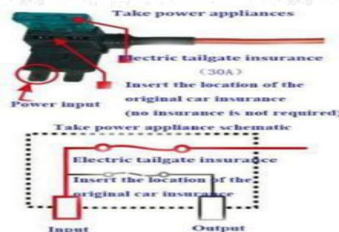
9.Fuse definition diagram
